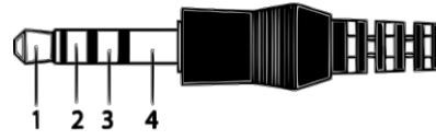
3.5mm Wiring Diagram
